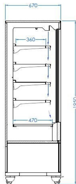
SECTION VIEW
